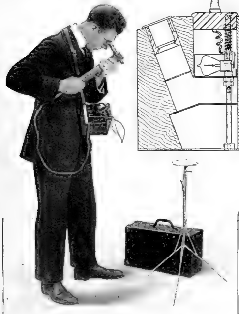
The aperture opposite the telescope is pointed toward the test-plate or any surface whose brightness is to be measured
